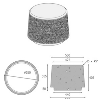
Ref: bollard 17 550x405mm
