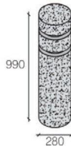
Ref: bollard 2 280x990mm
