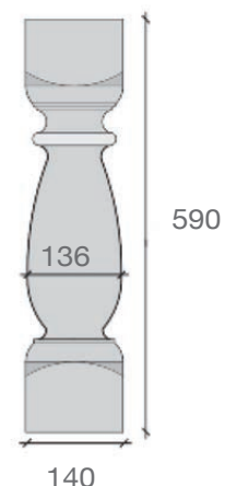
Ref: BALLUSTRADE 109 140 x 590mm
