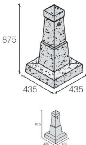
Ref: bollard 7 435x435x875mm
