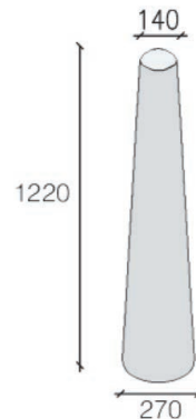
Ref: bollard 3 140x270x1220mm
