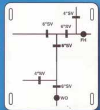
Schematic sign plates.
